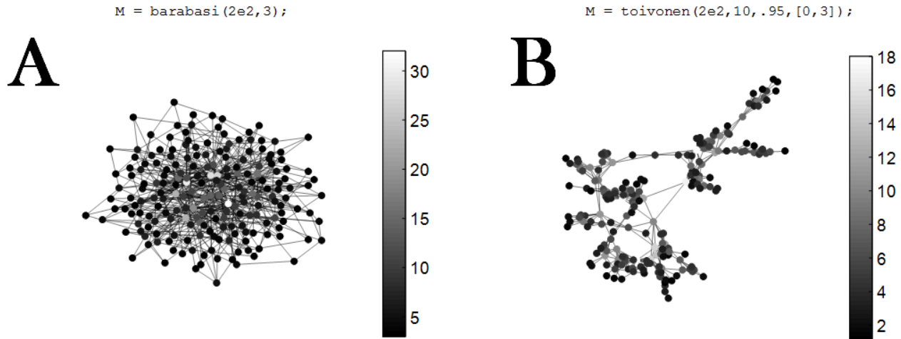
Figure 3 ■ Visualization of Barabasi (A) and Toivonen (B) Network in Matlab. Greyscale bar indicate degree k . Figure code can be obtained at https://osf.io/7apdm/ .
