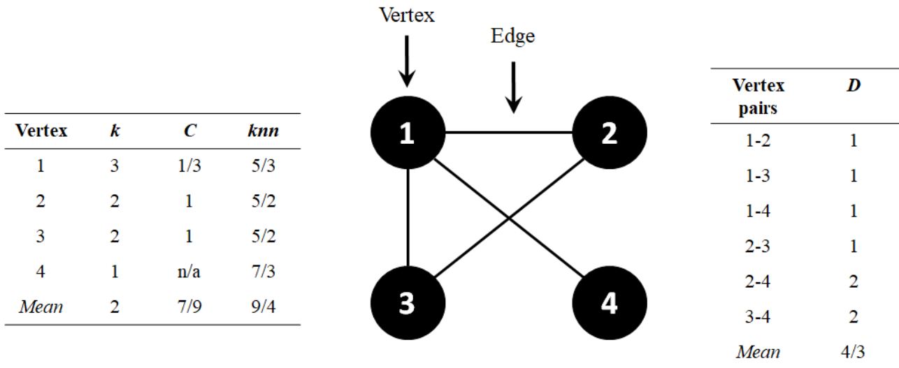
Figure 2 ■ In the middle is a small network consisting of 4 vertices (black circles) labelled 1 to 4. The lines connecting the vertices are undirected edges. The table to the left shows, for each vertex, the degree k , which is the number of edges connected to a vertex; the local clustering coefficient C , which is the proportion of possible edges that are actually present between the neighbors of a vertex; and k_{nn} , which is the average degree among the neighbors of a vertex. The table to the right shows the shortest distance D from one vertex to another for all vertex pairs, where each edge counts as a distance of 1. The mean of all quantities is shown at the bottom of the tables. By convention, the clustering coefficient C has no value (n/a = not available) for vertices with degree k < 2 , because in that case there are no possible edges between neighbors that can exist.
